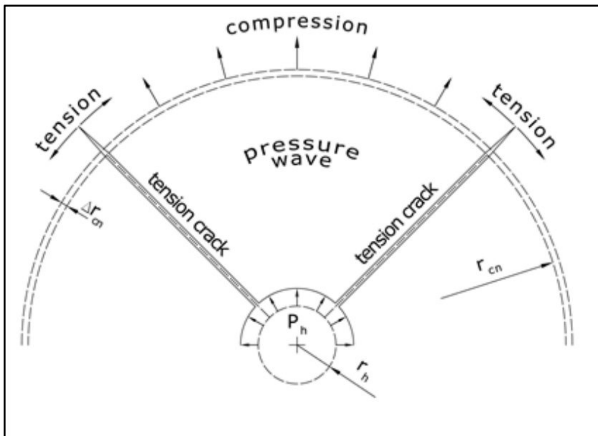
Figure 1 Schematic illustration of rock blasting model
