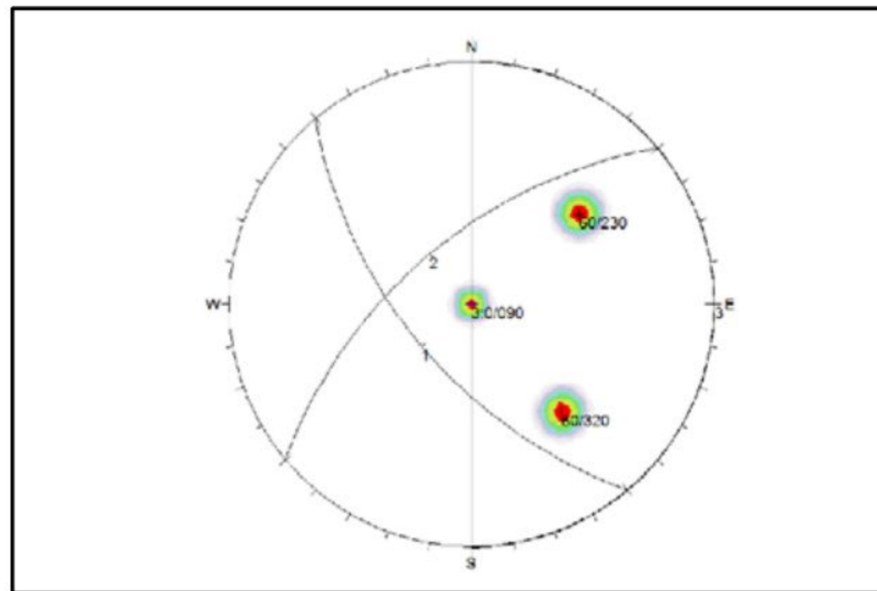
Figure 4 Preexisting and blast-induced joints orientation
