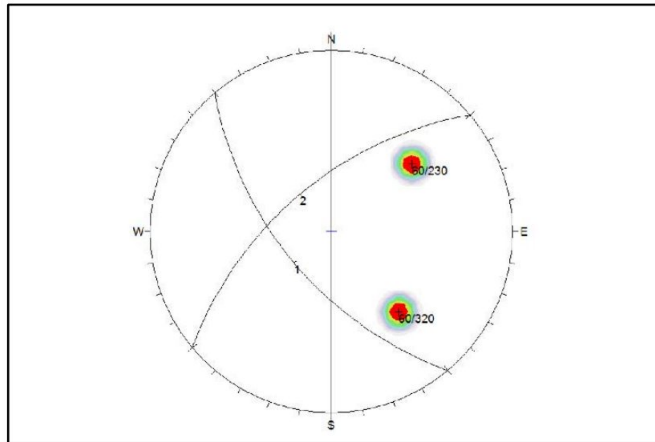
Figure 2 Preexisting joint sets in rock mass
