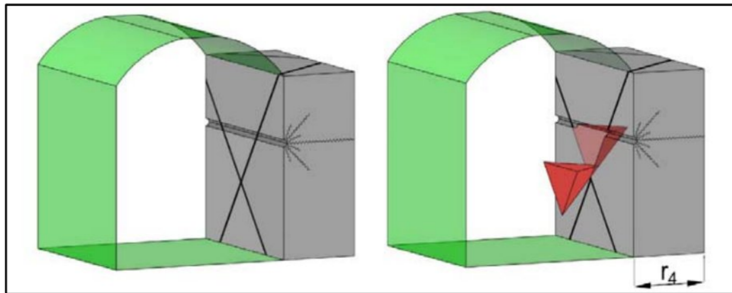
Figure 5 Unstable rock wedge formed in blasting process
