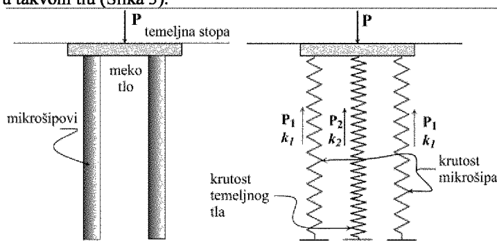
Slika 3. Kombinovani temelj – plitko fundirana stopa i mikrošipovi Figure 3. Combined foundation - shallow foundation and micropiles
