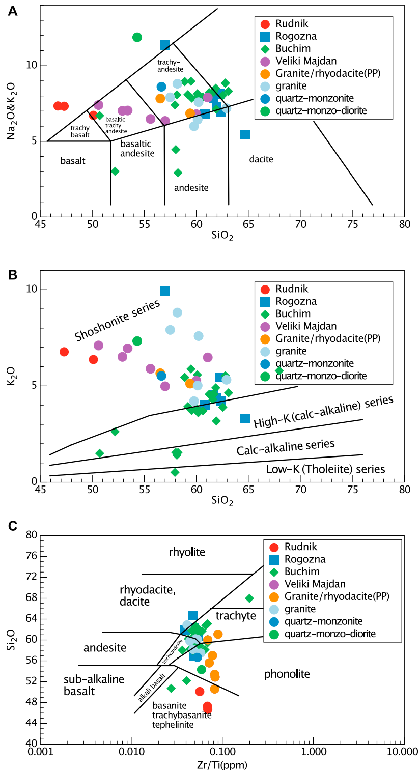
FIGURE 7 | Classification diagrams of whole-rock samples (results from XRF analyses). (A) Total alkalis versus silica (TAS) diagram (Le Maitre et al., 1989). (B) K_2O versus SiO_2 diagram, boundaries after (Rickwood, 1989). (C) SiO_2 versus Zr/Ti (ppm) for altered rocks after (Winchester and Floyd, 1976). Published data used for comparison are from Buchim (Lehman et al., 2013; green diamonds), Rudnik (Cvetković et al., 2006; red circles), Veliki Majdan (Prelevic, 2005; orange circles), and the Rogozna Mts (Borojević Šoštarić et al., 2012; blue squares).
